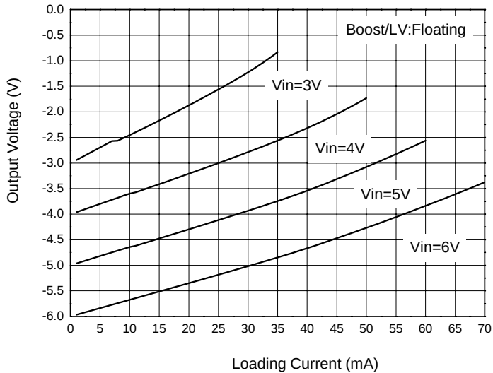
Fig. 1 Output Voltage vs. Load Current
