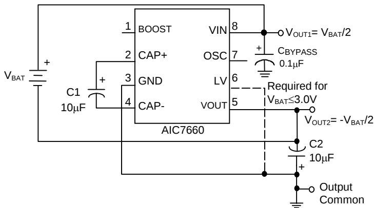
Fig. 18 Battery Splitter
