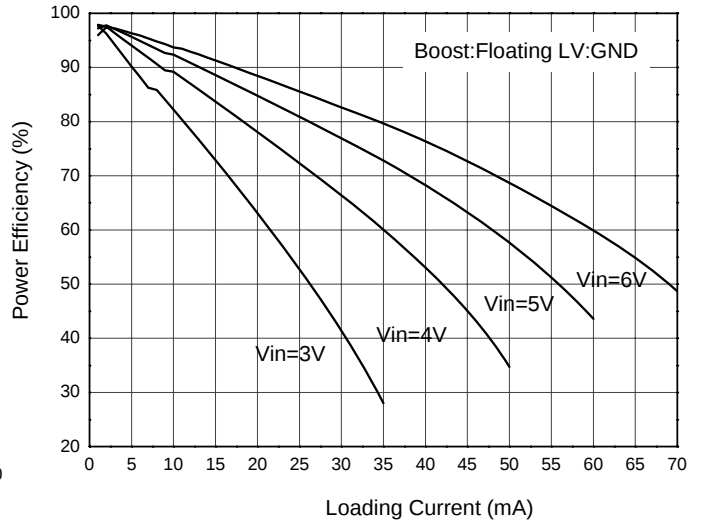
Fig. 8 Power Efficiency vs. Load Current
