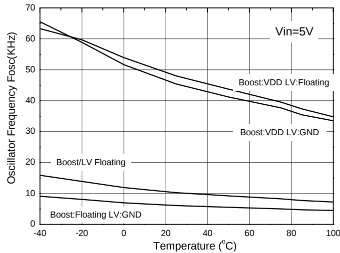
Fig. 13 Oscillation Frequency vs. Temperature
