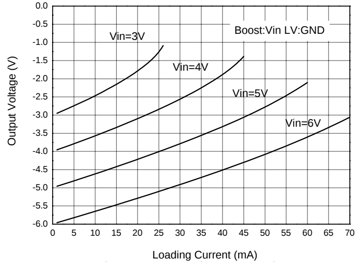
Fig. 2 Output Voltage vs. Load Current
