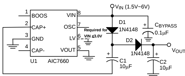
Fig. 16 Voltage Doubling
