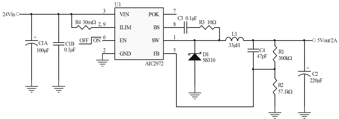
Fig. 6 AIC2972 Application Circuit for 5V/2A Output Application
