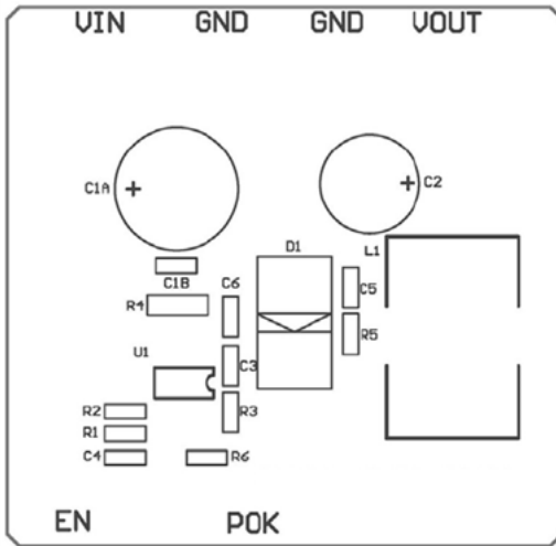
Fig. 5 Top Component Placement
