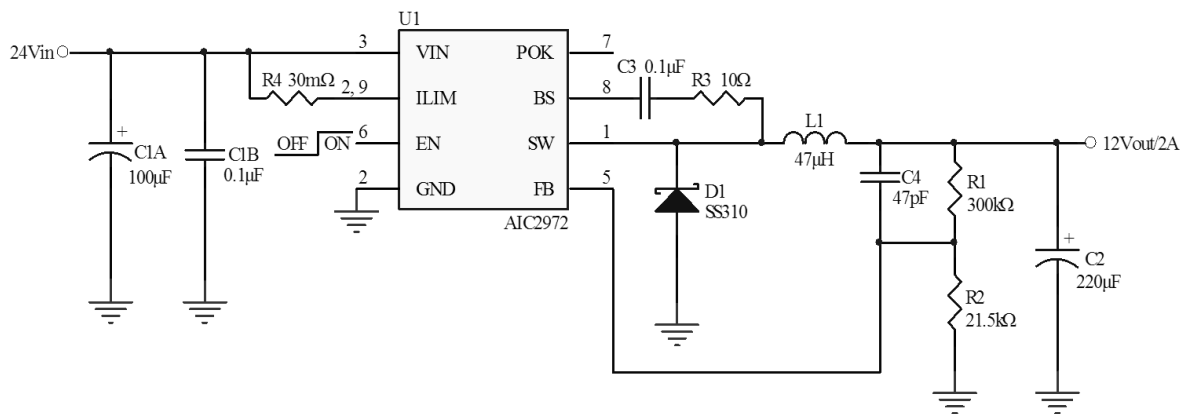
Fig. 7 AIC2972 Application Circuit for 12V/2A Output Application
