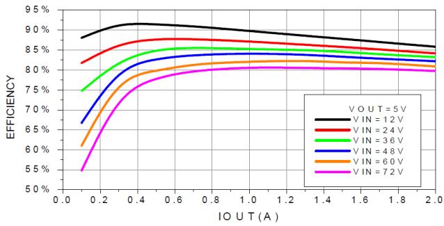
Fig. 1 Efficiency vs. Output Current
