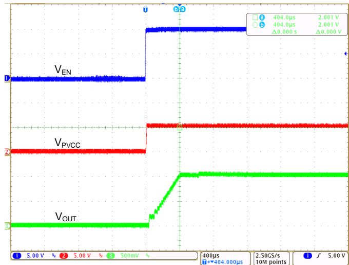
Fig. 10 Star_Up at V_{IN}=12V , V_{OUT}=1.05V , I_{OUT}=0A
