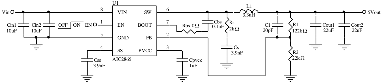
Fig. 11 Application Circuit for V_{IN} \geq 14V Condition
