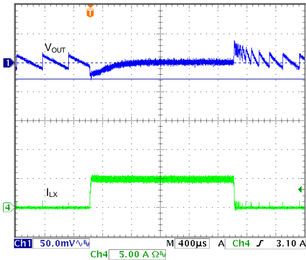
Fig. 9 V_{IN}=12V , V_{OUT}=1.05V , I_{OUT}=0A to 5A
