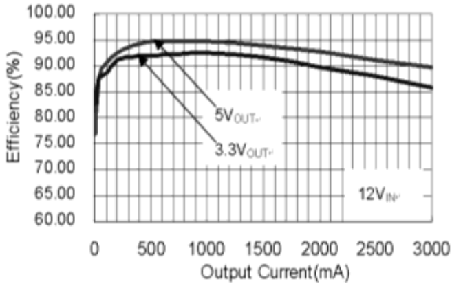
Fig. 1 Efficiency vs. Load Current
