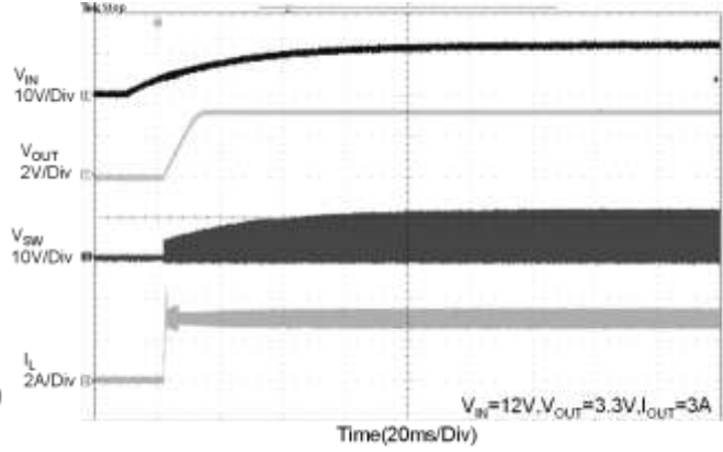
Fig. 2 Start-Up Waveform at V OUT =3.3V, I OUT =3A
