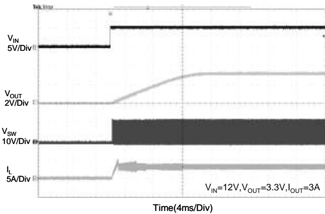
Fig. 3 Start-Up Waveform at V OUT =3.3V, I OUT =3A
