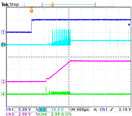
(CH1: V_{EN} , CH2: V_{LX} , CH3: V_{OUT} , CH4: I_L )
