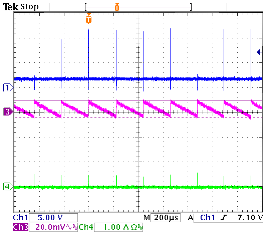
(CH1: V_{LX} , CH3: V_{OUT(ac)} , CH4: I_L )
