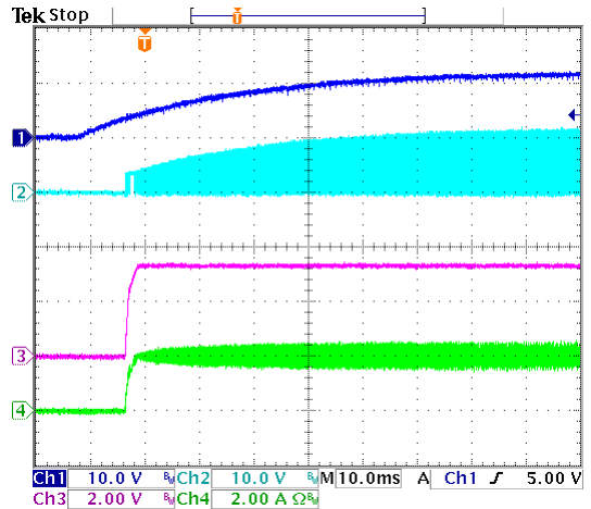
(CH1: V_{IN} , CH2: V_{LX} , CH3: V_{OUT} , CH4: I_L )
