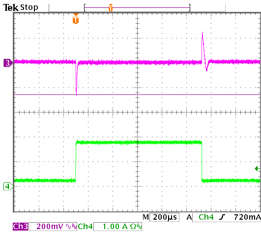
(CH3: V_{OUT(ac)} , CH4: I_{OUT} )
