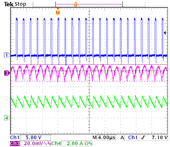
(CH1: V_{LX} , CH3: V_{OUT(ac)} , CH4: I_L )
