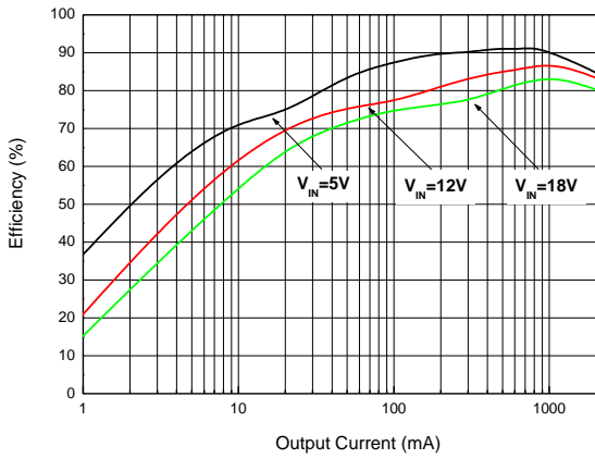
Fig. 1 Efficiency vs. Output Current ( V_{OUT}=1.8V )
