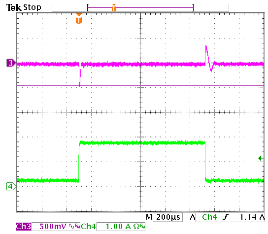
(CH3: V_{OUT(ac)} , CH4: I_{OUT} )
