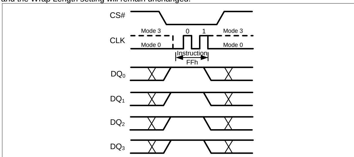
Figure 59 Disable QPI Instruction (QPI Mode only)
