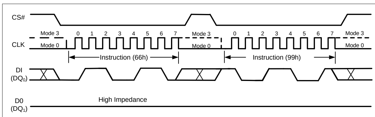
Figure 60 Enable Reset and Reset Instruction Sequence (SPI Mode)
