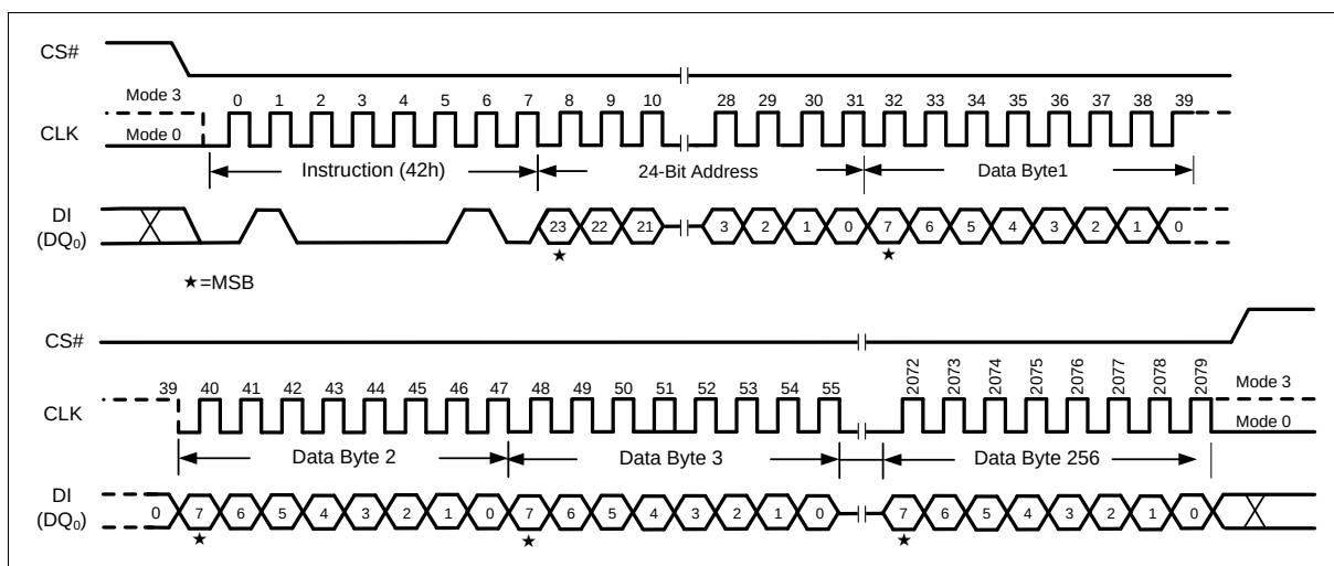
Figure 54 Program Security Sectors Instruction (SPI Mode only)
