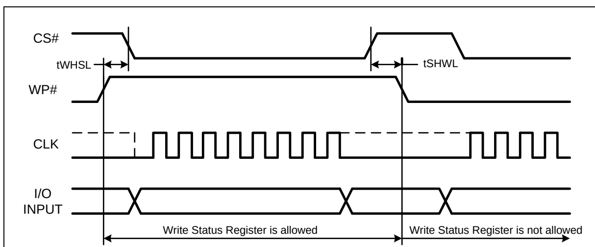
Figure 67 WP# Timing
