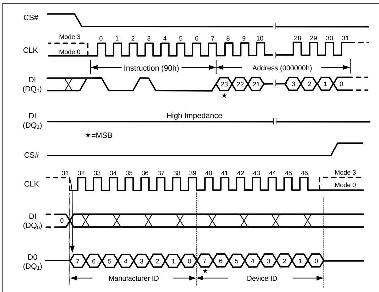
Figure 45 Read Manufacturer / Device ID Instruction (SPI Mode)
