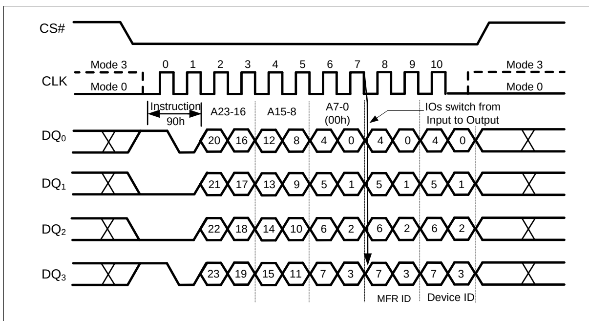
Figure 46 Read Manufacturer / Device ID Instruction (QPI Mode)
