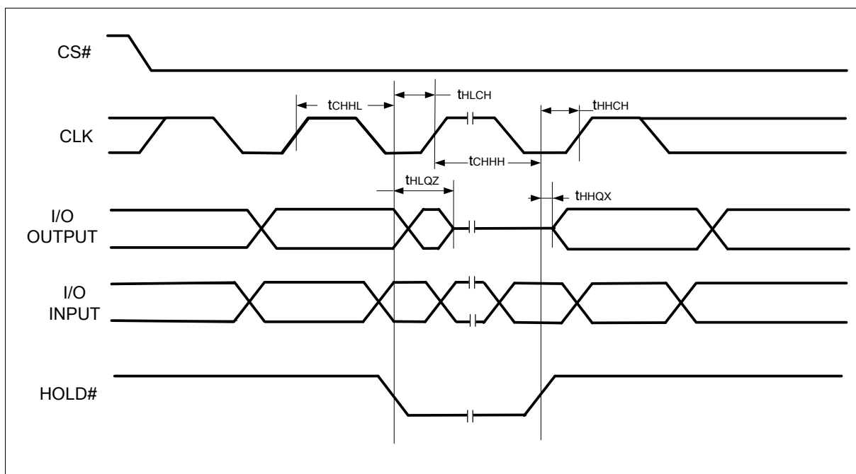
Figure 66 Hold Timing
