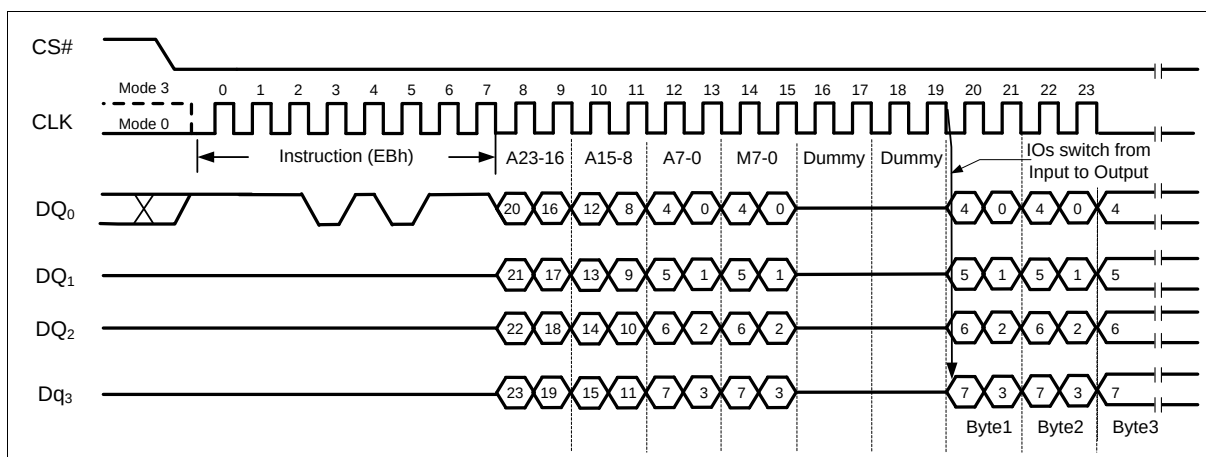
Figure 21 Fast Read Quad I/O Instruction (Initial instruction or previous M5-4#10, SPI Mode)
