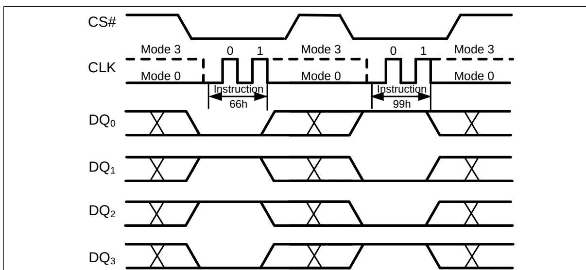
Figure 61 Enable Reset and Reset Instruction Sequence (QPI Mode)
