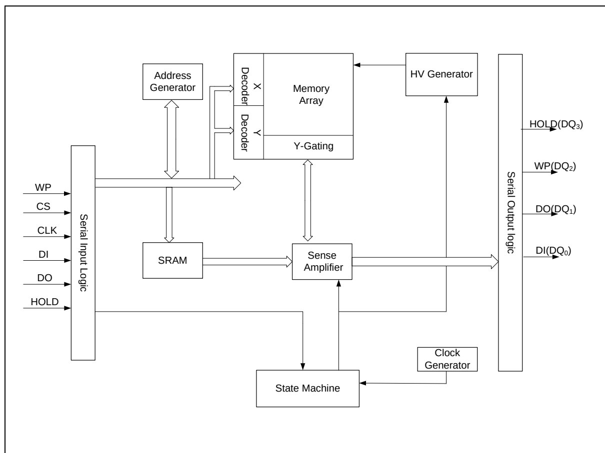
Figure 1 FM25W04 Serial Flash Memory Block Diagram
